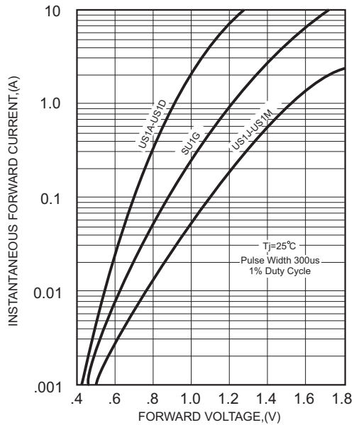
FIG.1-TYPICAL FORWARD CHARACTERISTICS
